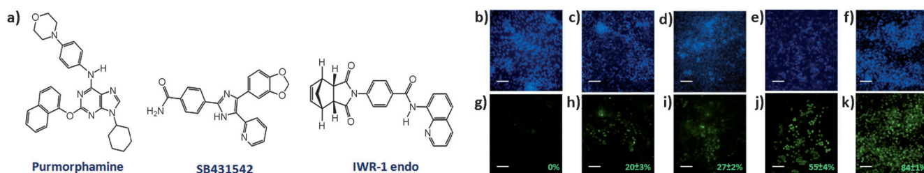
Figure 3. a) Structure of the three small molecules that efficiently induce Nkx2.5 expression from hESCs-derived primitive streak cells. b–k) Immunofluorescent images of hESC-H9-derived primitive streak cells that were treated with either 0.1% DMSO (b,g), SB431542 (5 \mu M) (c,h), Purmorphamine (5 \mu M) (d,i), IWR-1 endo (5 \mu M) (e,j), or a chemical cocktail consisting of IWR-1 endo (5 \mu M), purmorphamine (5 \mu M), and SB431542 (5 \mu M) (f,k) in CDM. Fluorescent images were then analyzed with an Opera high-content confocal imaging system to quantitate the percentages of Nkx2.5-positive cells (green). Values are the mean \pm s.d. for three measurements. (Scale bar, 100 \mu m.)
